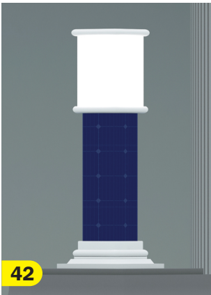
Article Code : FORTUNE (24S002) Light Source : Led 6w Height : 522 mm Solar Pannel : Mono Perc 15w CCT : 3500k-NDL/6000k-CDL
