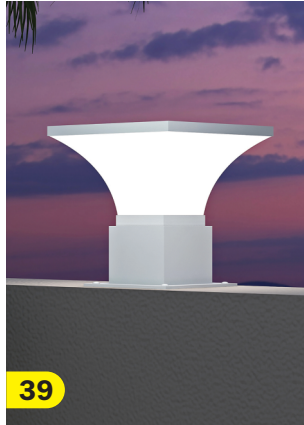
Article Code : FORTUNE (24S005) Light Source : Led 10w Height : 250 mm Solar Pannel : Mono Perc 8w CCT : 3500k-NDL/6000k-CDL
