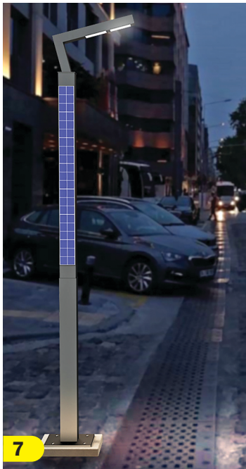
Article Code : LINELIT (24S026) Light Source : Led 20w Height : 2400 mm Solar Pannel : Mono Perc 84w CCT : 3500k-NDL/6000k-CDL
